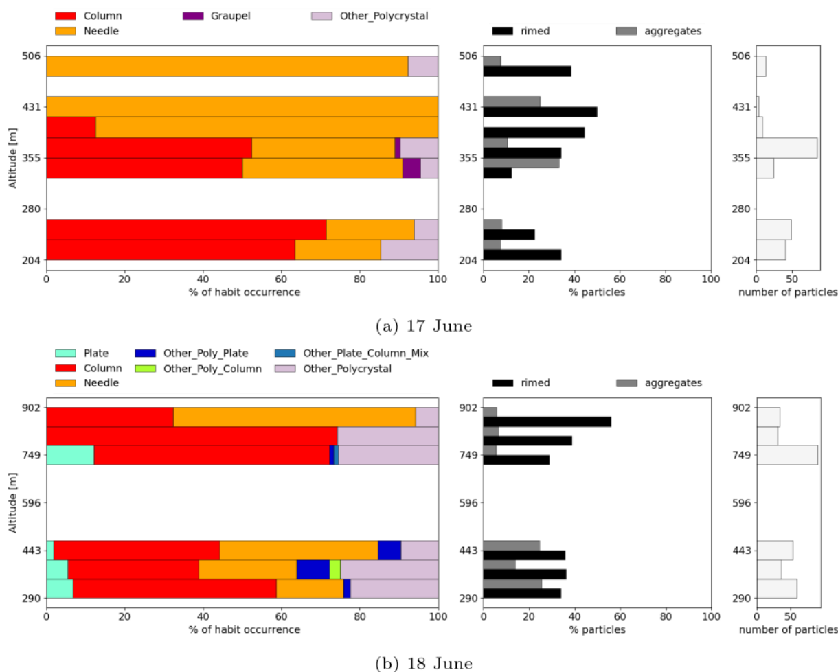
Figure 11. Analysis of ice crystal habits during cloud sampling on 17 and 18 June during the normal period.
