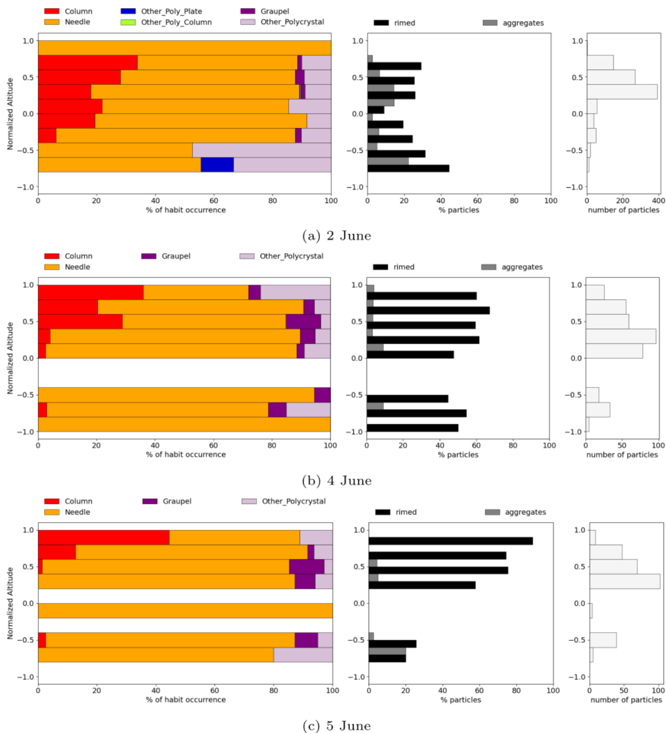
Figure 8. Analysis of ice crystal habits imaged by the PHIPS during cloud sampling on 2, 4 and 5 June during the warm period.
