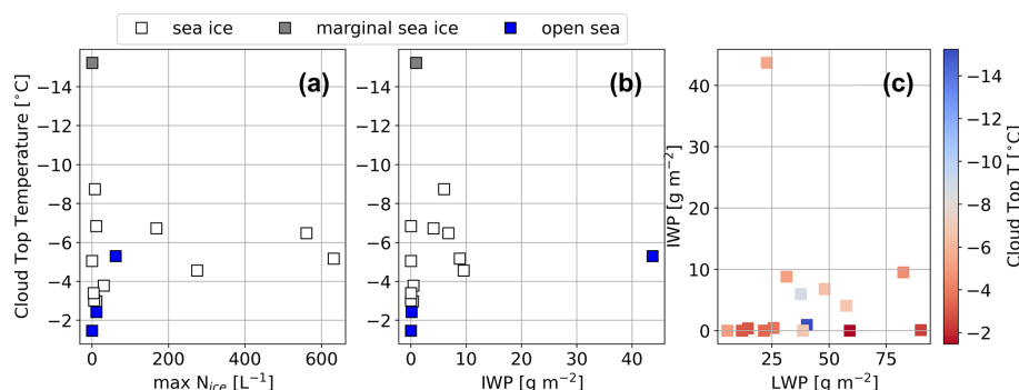
Figure 14. Maximum 10 s ice crystal number concentration ( N_{\text{ice}} ; panel a ) and ice water path (IWP; panel b ) as a function of cloud top temperature during ACLOUD for vertical cloud profiles over pack ice (white symbols), marginal sea ice zone (grey symbols) or the open-sea surface (blue symbols). The correlation between liquid water path (LWP) and IWP is shown in panel (c) , where the symbols are colour-coded with the cloud top temperature. The list of vertical cloud profiles can be found in the Supplement.
