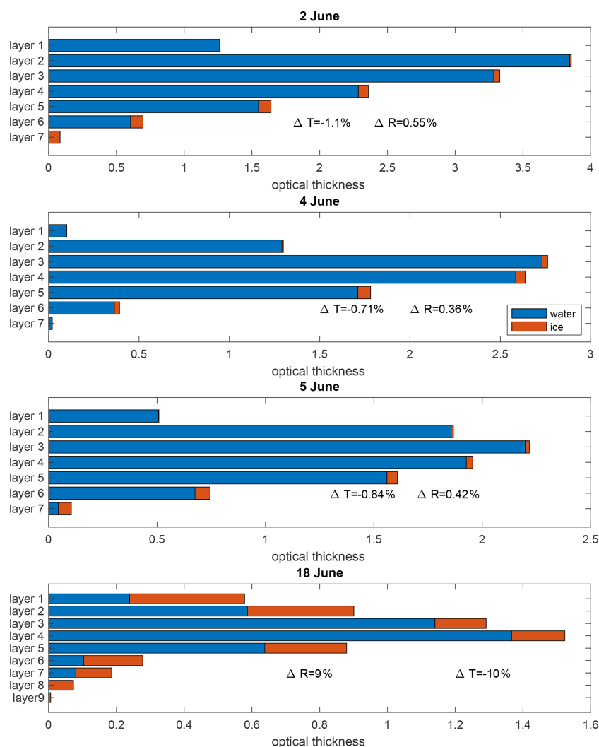
Figure 13. The optical thickness for liquid and ice phase for different altitudes within the cloud. The difference in albedo ( \Delta R ) and transmissivity ( \Delta T ) is calculated for modified simulation, where the ice phase is treated optically like the liquid phase.
