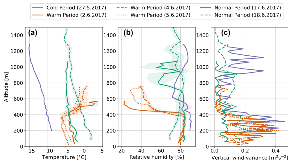
Figure 2. Average temperature (a), relative humidity with respect to water (b) and vertical wind variance (c) for the vertical profiles performed during the cold period (blue), warm period (red) and normal period (green). Note that the lines represent the average values during the entire cloud sampling period. The shaded area in panels (a) and (b) shows the standard deviation. Note that the absolute value of relative humidity is not considered to be reliable, and the values in panel (b) should only be considered to represent the trend in the relative humidity.
