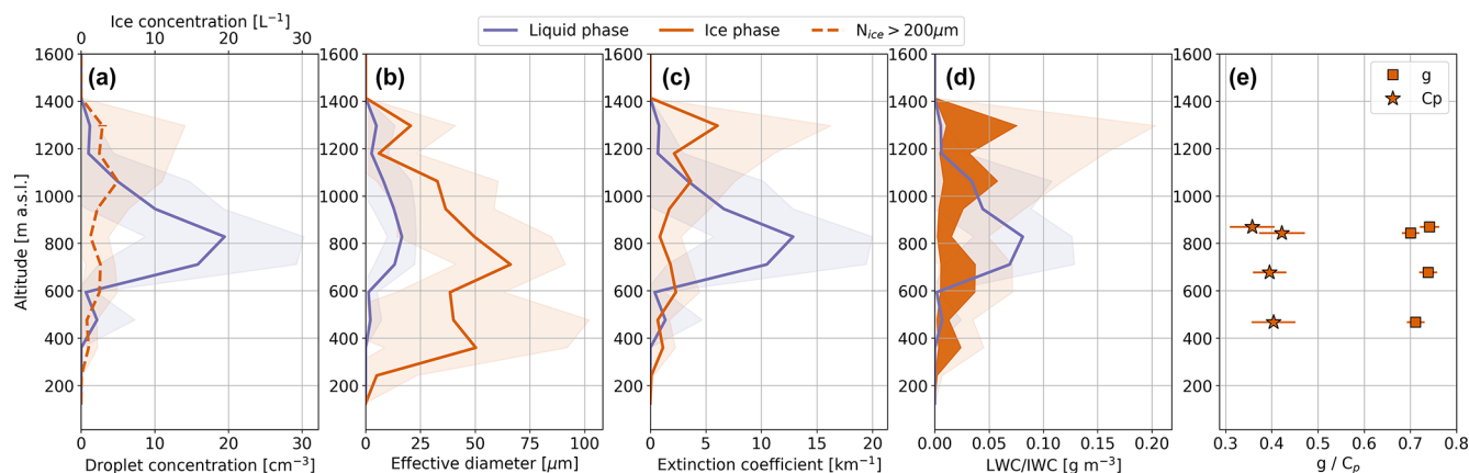
Figure 12. Vertical profile of average droplet number concentration (a), effective diameter (b), extinction coefficient (c) and condensed water content (LWC/IWC) (d) performed on 18 June over the open ocean during the normal period. The shaded area illustrates the standard deviations. The horizontal error bars in panel (a) illustrate the statistical uncertainty in N_{\text{ice}>200\mu\text{m}} calculated using \sigma(N_{\text{ice}>200\mu\text{m}})/\sqrt{n} , where n is the number of counts included in calculation of the mean concentration. In panel (d) the dark shaded area illustrates the range in IWC when using M – D relations of BF95 (upper limit) and a habit-dependent M – D relation of Lawson and Baker (2006) for needles (lower limit). The 10 s average measurement data were binned in altitude bins with bin width of 117 m for calculating the statistics. Cloud sampling was performed between 78.2.1 and 78.3° N and 5.2 and 9.9° E.
