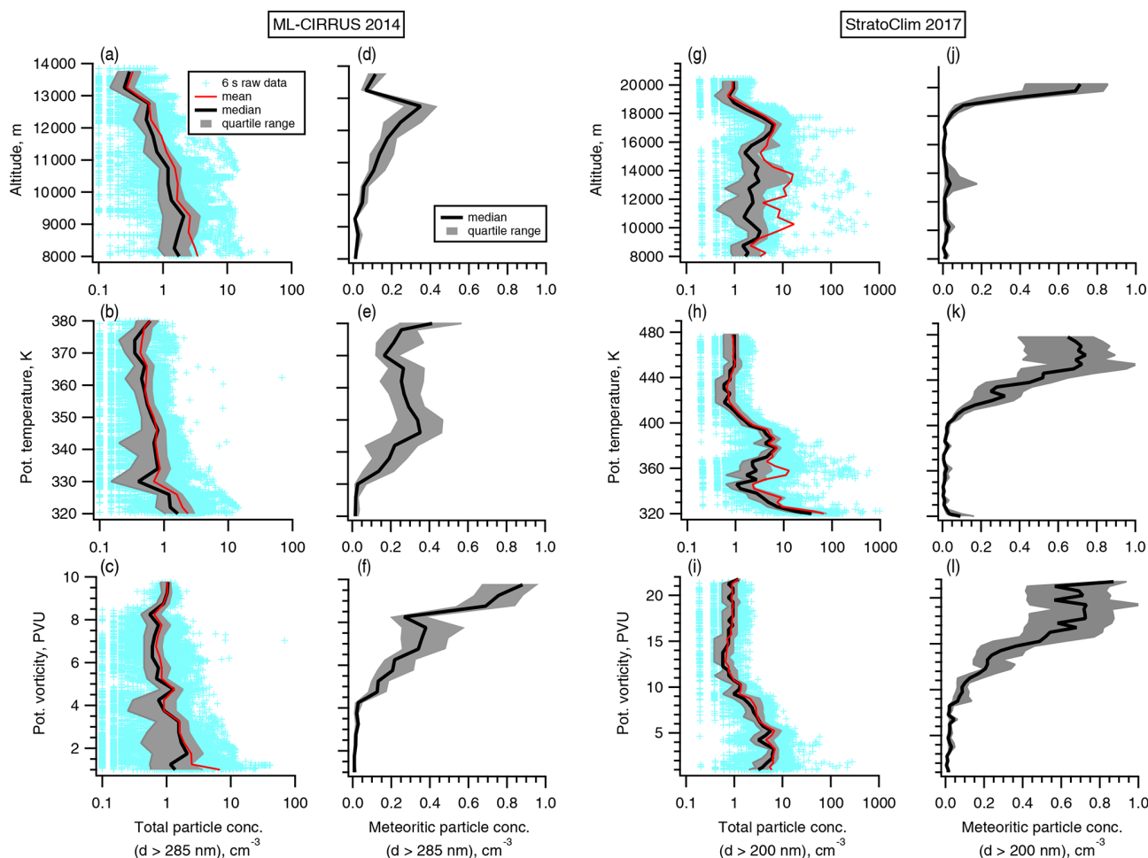
Figure 7. Total particle number concentrations measured during ML-CIRRUS 2014 ( d_{ve} > 285 nm, a–c ) and StratoClim 2017 ( d_{ve} > 200 nm, g–i ) along with calculated number concentrations of particles containing meteoric material (ML-CIRRUS 2014: d–f ; StratoClim 2017: j–l ). Data are shown for the upper troposphere and lower stratosphere (altitude > 8 km, potential temperature > 320 K, PV > 1 PVU). Light-blue markers: 6 s raw data; red line: mean; black line: median; grey area: quartiles (25 % and 75 %).
