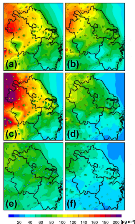
Figure 3. Spatial comparisons of hourly-averaged concentrations of simulated and constrained PM 2.5 with surface observations across the YRD for January 2016 (a, b), January 2019 (c, d), and the G20 summit (e, f): (a) NO_2016; (b) DA_2016; (c) NO_2019; (d) DA_2019; (e) NO_G20; (f) DA_G20. Circles denote ground measurement sites.
