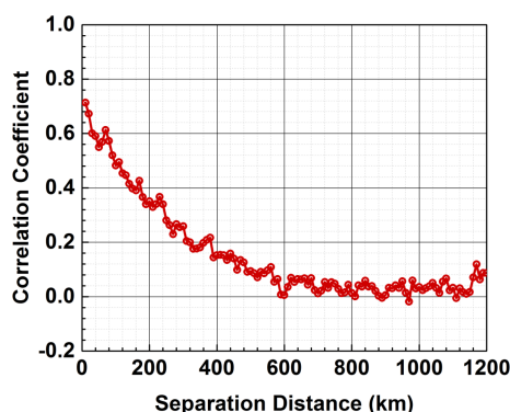
Figure 2. Correlation coefficients (averaged over 10 km) as a function of the separation distances between two surface-level monitoring stations using the Hollingsworth–Lönnberg method.
