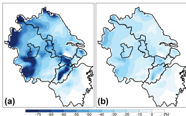
Figure 9. (a) Spatial distributions of the PM 2.5 mitigation potential across the YRD and (b) their differences with the impacts of long-term emission control strategies from 2016 to 2019 (Fig. 5f). Both spatial patterns of long-term emission control strategy impacts (Fig. 5f) and the localized PM 2.5 mitigation potential in the main urban areas of Hangzhou (Fig. S10), with the proportion calculator, result in panel (a).
