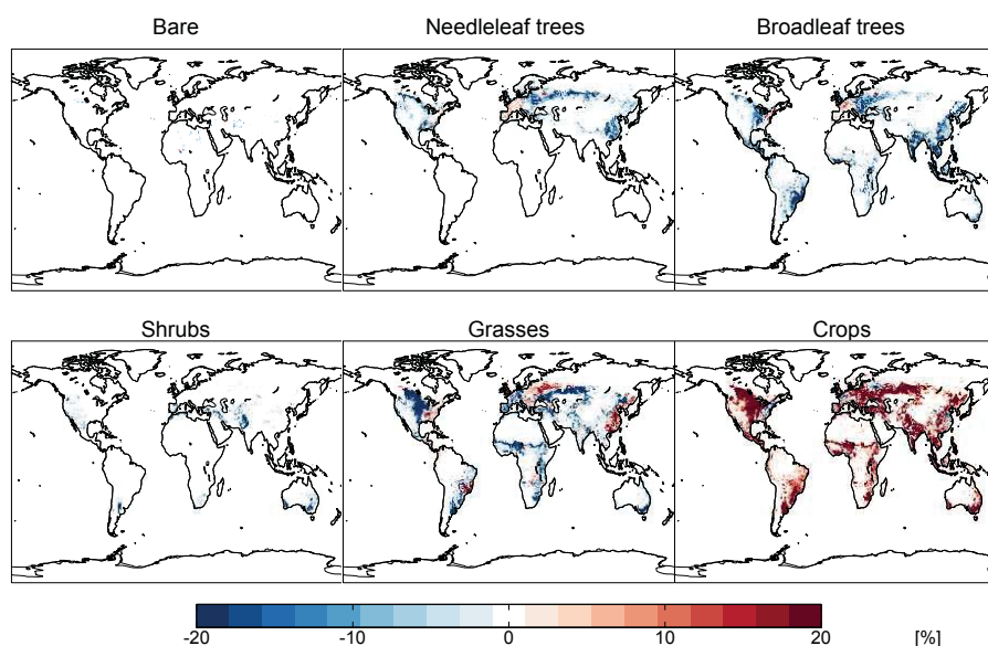
Figure 2. Change from preindustrial (1850) to present day (2000) in the percentage of land area occupied by six classes of vegetation.
